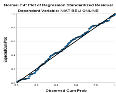
Gambar 1. Uji Normalitas P-P Plot
