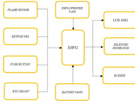
Gambar 3.1 Blok Diagram
