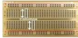
Gambar 5 Breadboard
