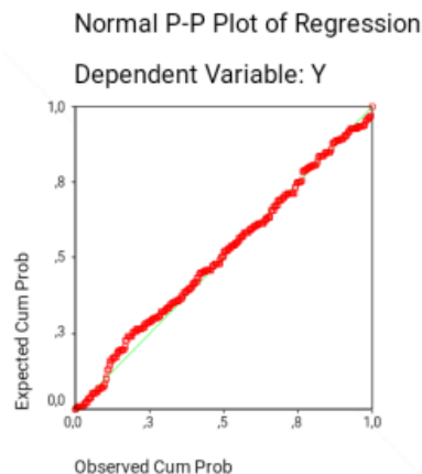
Figure 2. Normal Distribution Plotting
