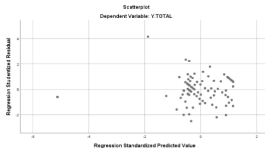
Gambar 4.2 Scatter Plot
