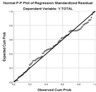
Gambar 4.1 Normal P-Plot
